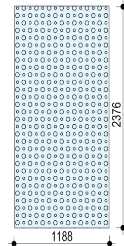
Alternating Circular 12/20/66 R
