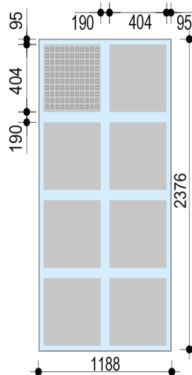
Standard Square Type B8 - 8/18Q
